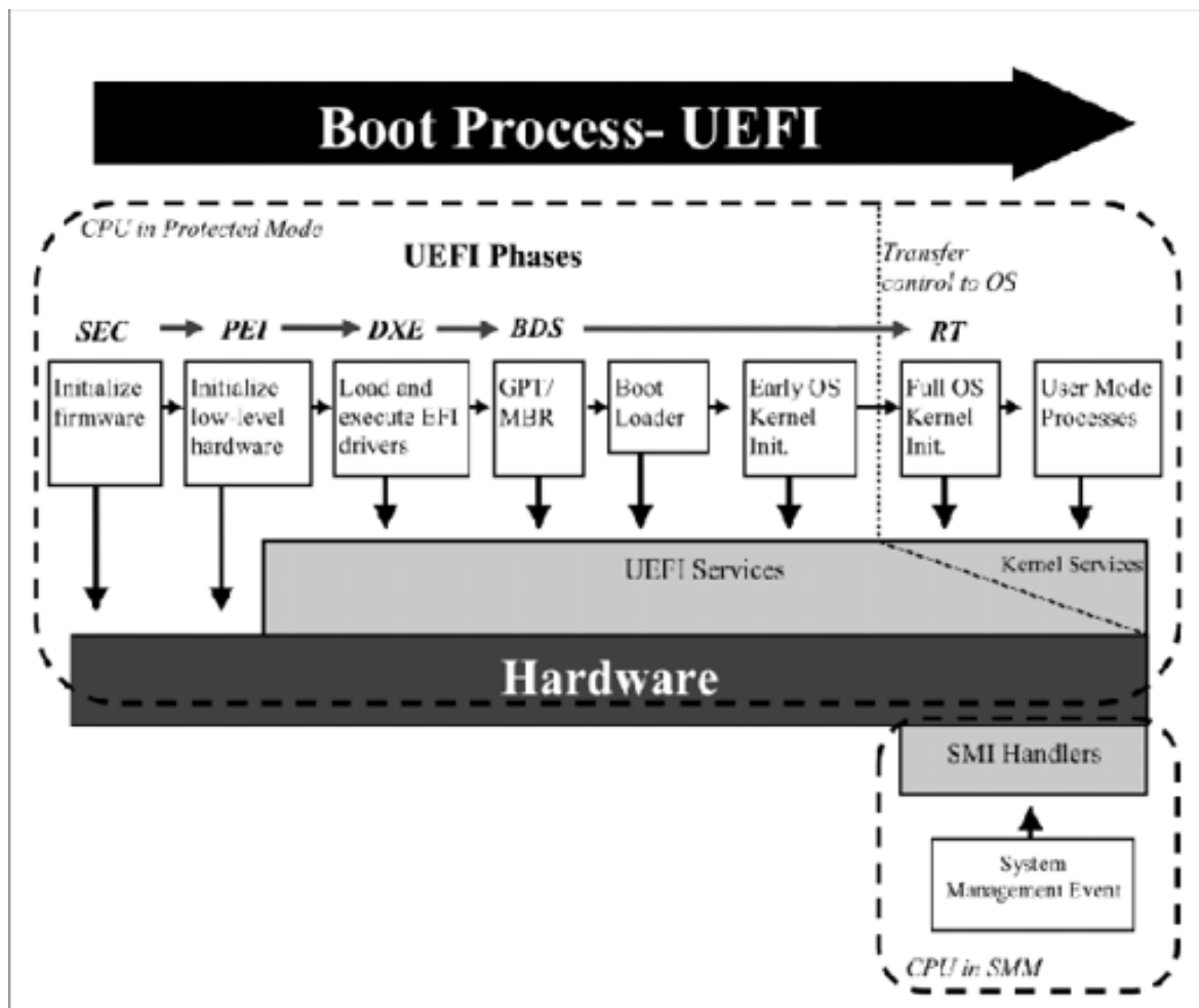
Figure 2: UEFI BIOS Boot Process
